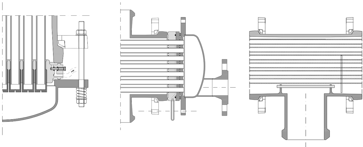
Option OST1: Drainage/ventilation when installed vertically
